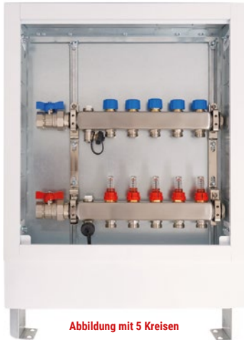
VA-FBif - TT-AGEw 1" - 110T
